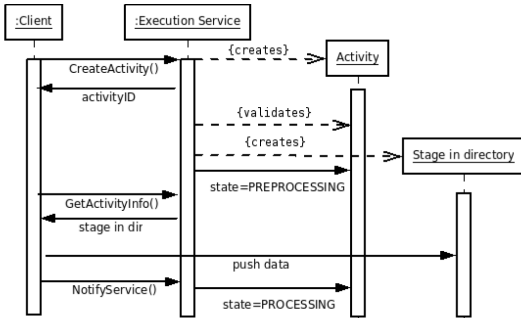
Figure 3: Activity creation, validation and client data push
