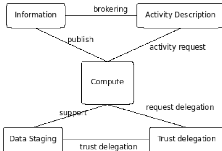
Figure 1: Relationship between execution service elements
