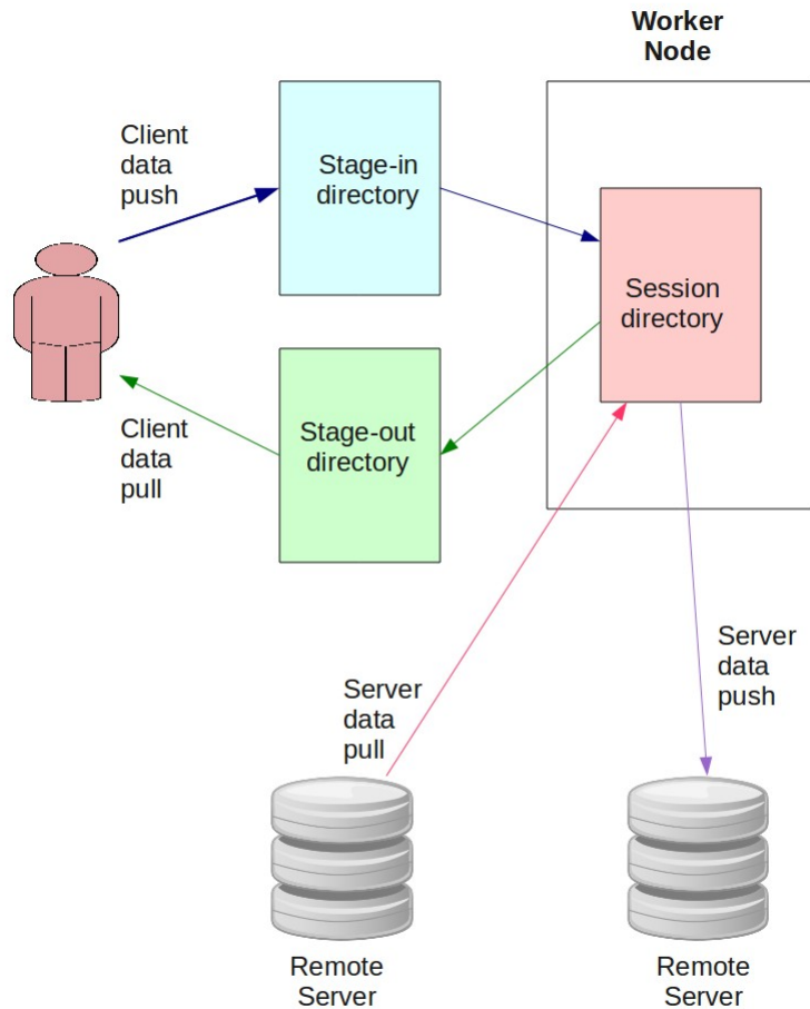
Figure 2: Data staging: directories and actors
